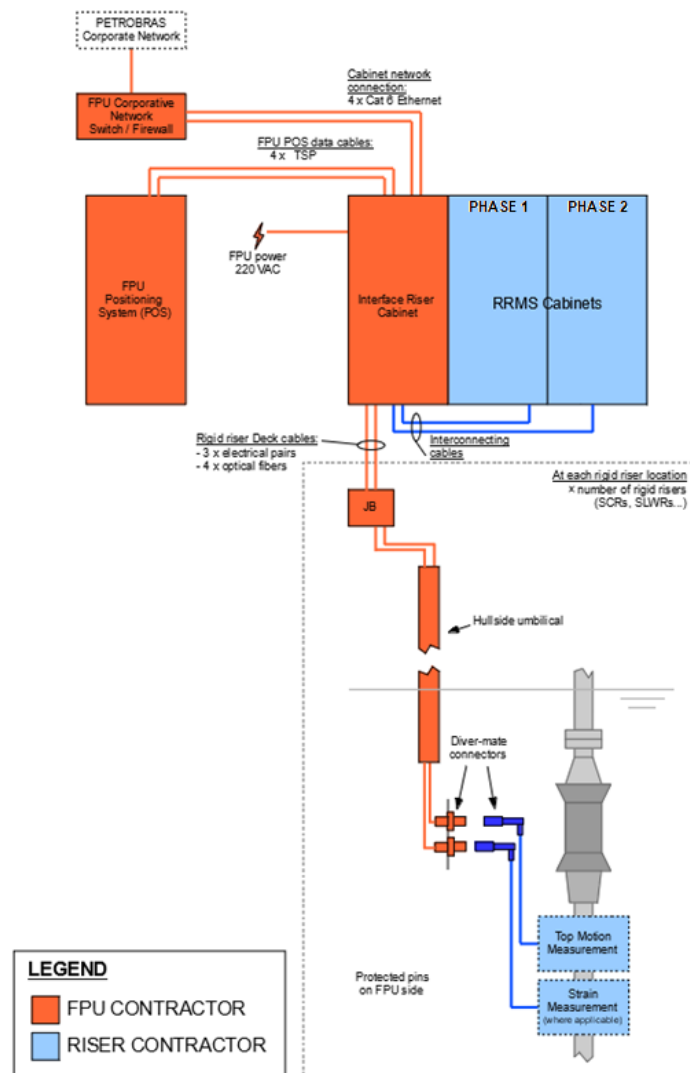
Figure 4 — General topology – RRMS System (for Phases 1 and 2)
