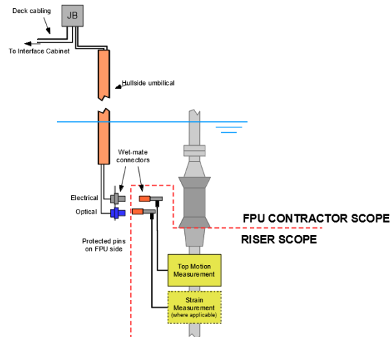
Figure 11 — Rigid riser connection scheme
