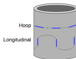
Figure 7 — Schematic view of strain sensing around riser pipe (only active sensors shown)
