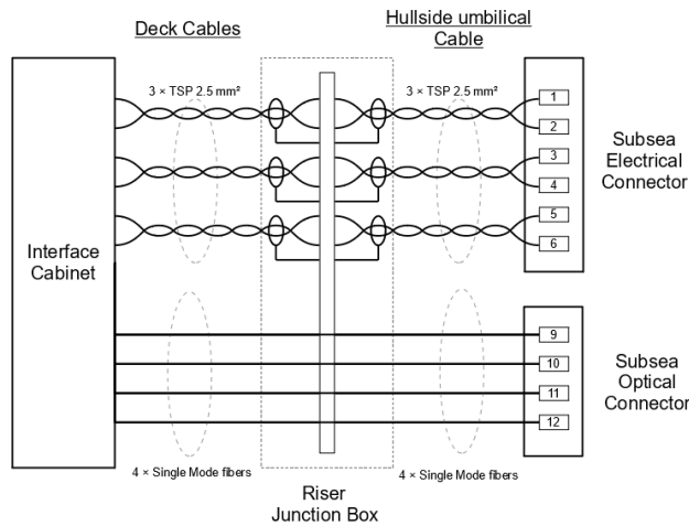
Figure 10 — Connection diagram for rigid riser cabling
