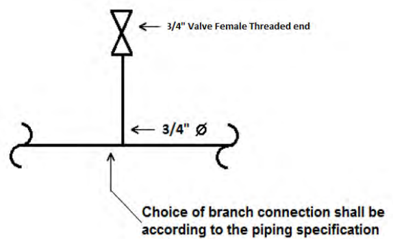
Figure C.6 – Threaded end valve
