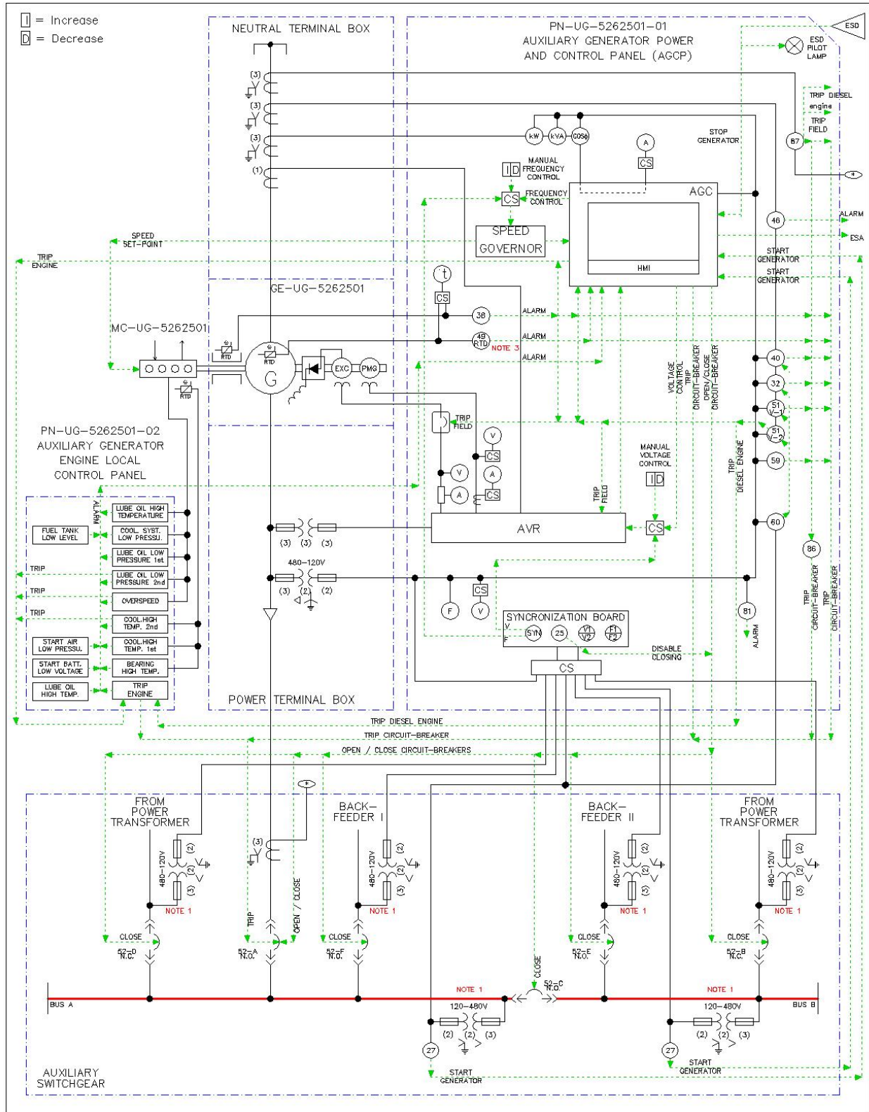
Figure 1 - Typical Protection and Communication Diagram – Isolated System
