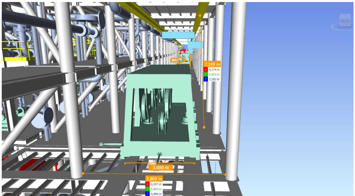
Figure 2: Trolley Area Limitation – dimensions.
