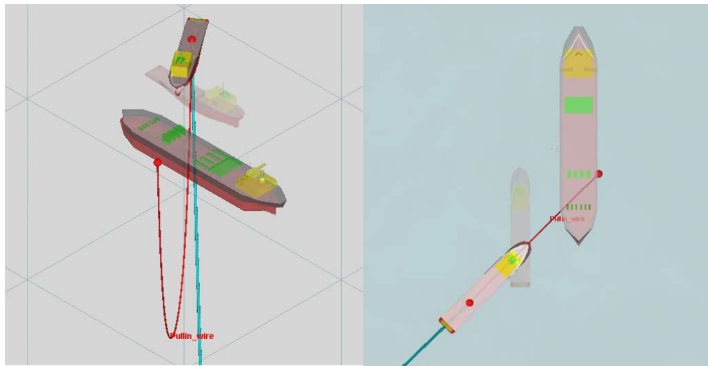
Figure 5: Riser pull-in via keelhauling with starboard approaching.
