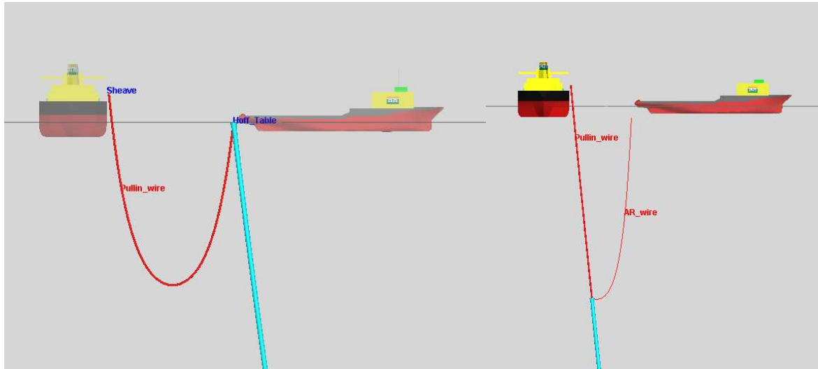
Figure 4: Direct riser pull-in with portside approaching.
