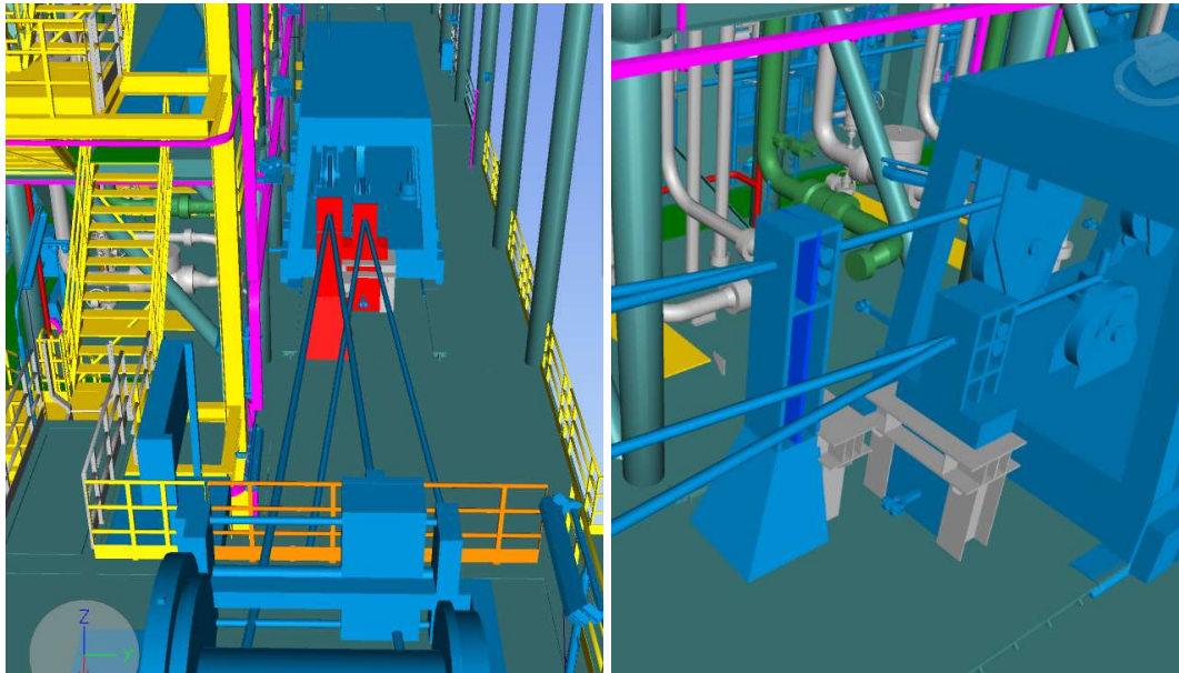
Figure 7: Main and auxiliary wire rope centralizers.
