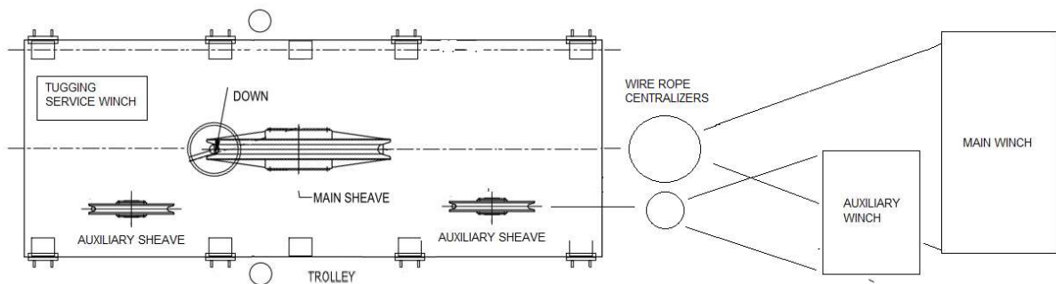
Figure 6: Schematic pull-in system.
