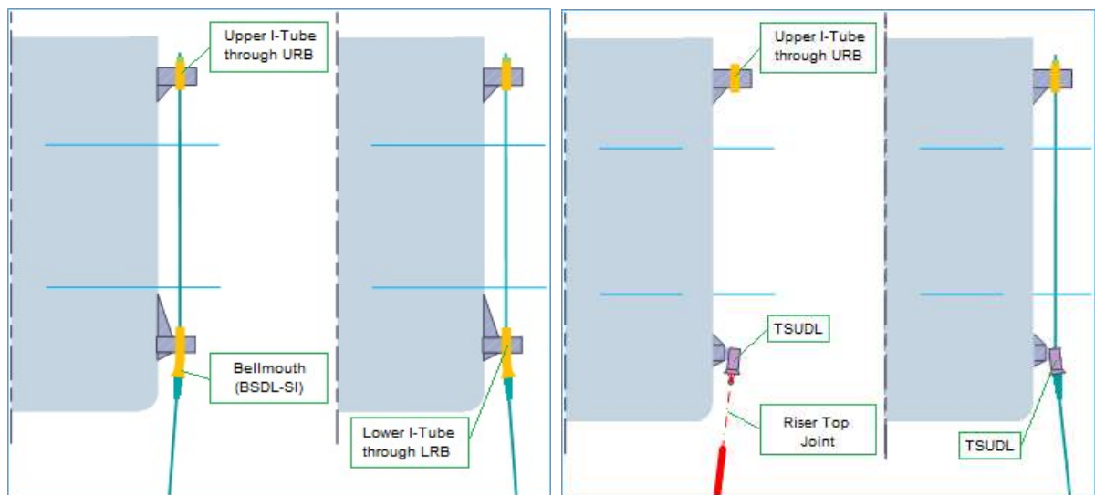
Figure 3: Riser Balcony Configuration.
