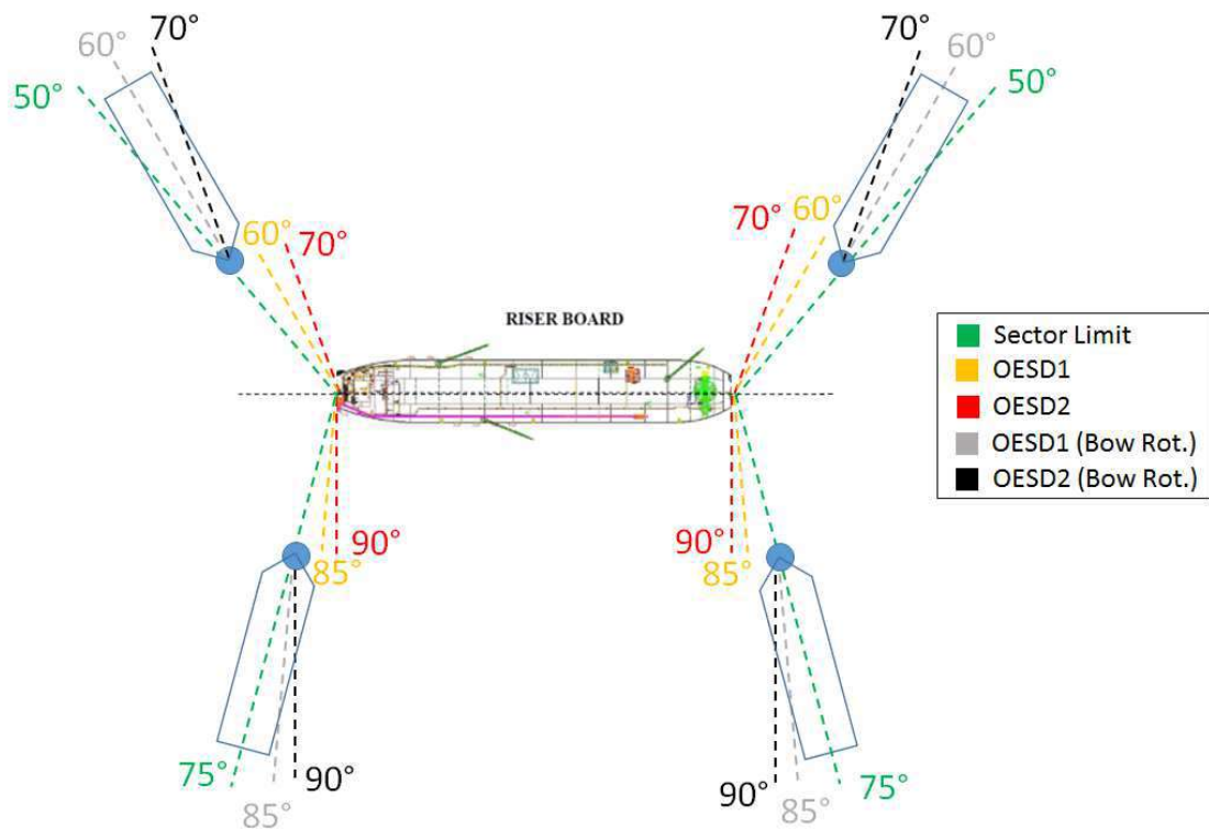
Figure 10-1 – Spread Mooring FPSO.
