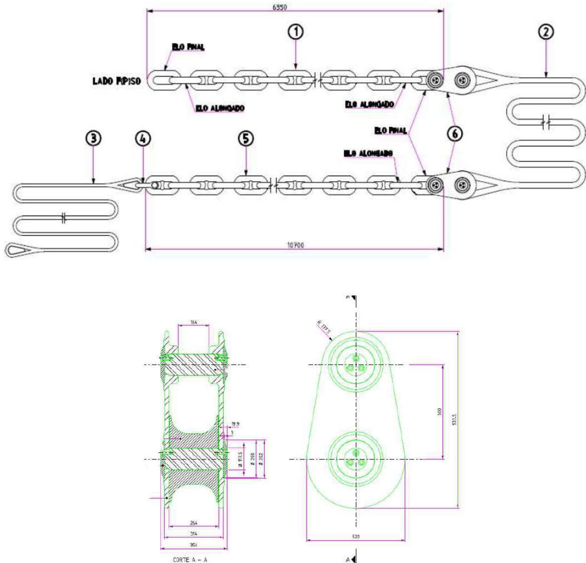
Figure 5-1– Rope-chain conector.
