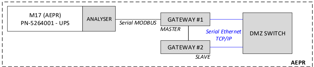
Figure 4: schematic interconnections
