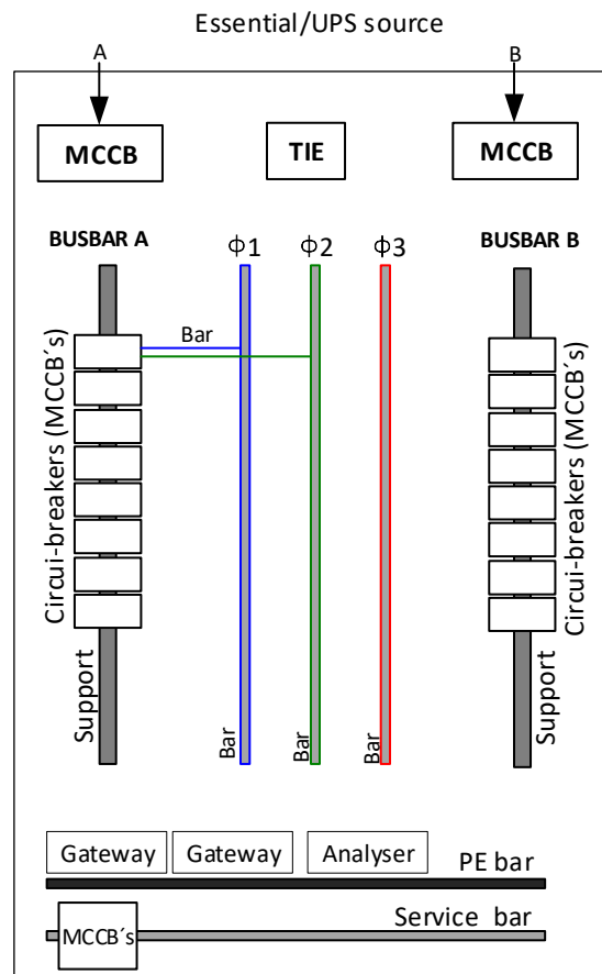
Figure 1: typical internal AC panel arrangement
